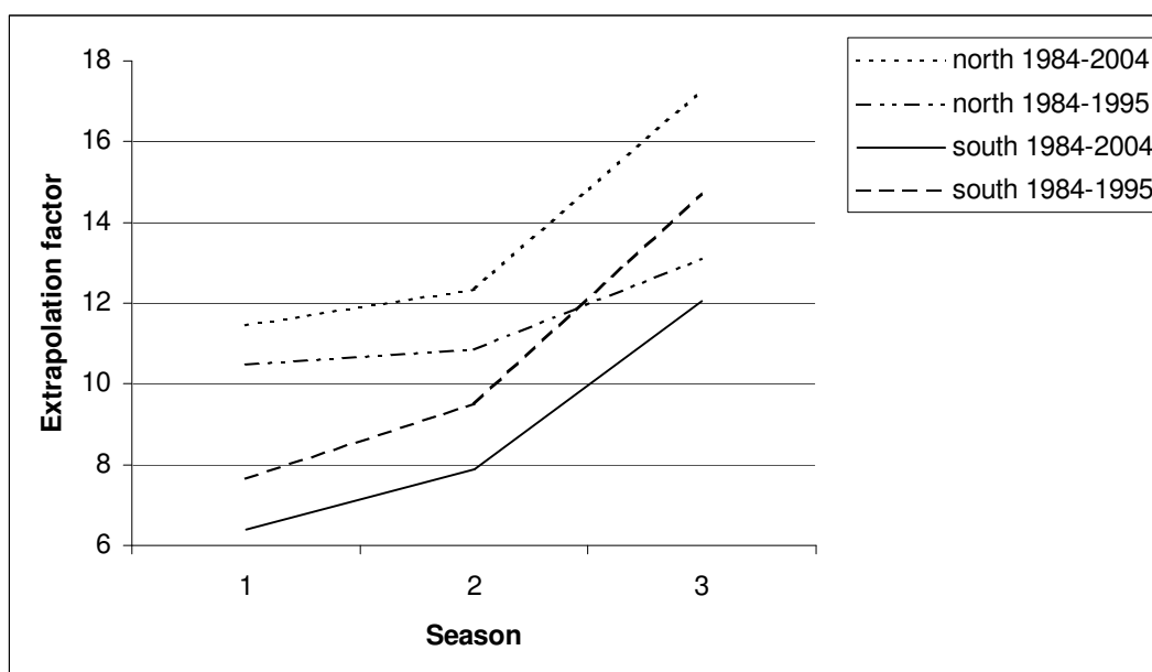
Fig. 2. Extrapolation factors (from Swenson and Katajisto 2005, their Fig 1) used to calculate the total number of brown bears that correspond to one reproduction, depending on the study period, study area, and season of the year in Sweden . Seasons are: 1) early spring after denning, 2) midsummer after the mating season, and 3) late autumn prior to denning. This figure is only for illustrative purposes, as these extrapolation factors are not valid for Norway.
